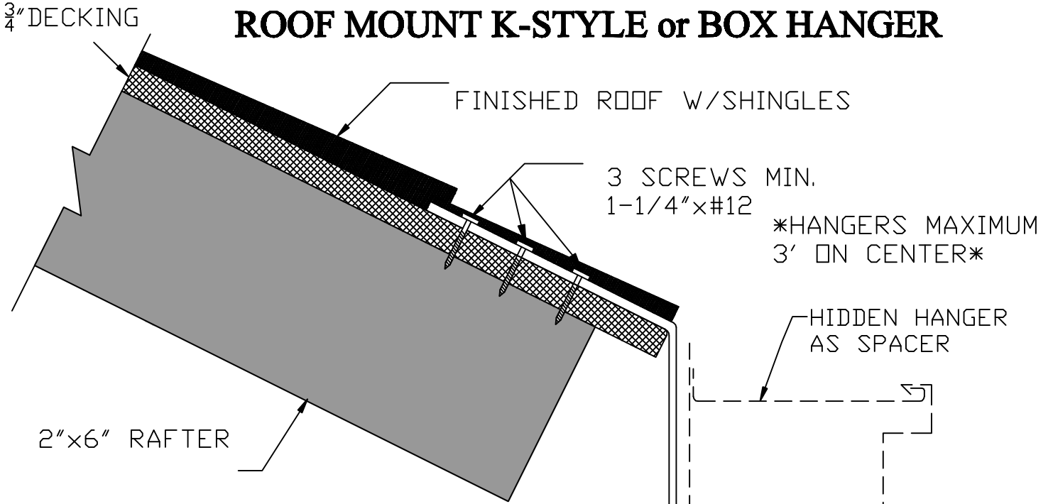
TYPICAL PROFILE K-STYLE GUTTER
