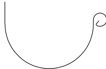
TYPICAL GUTTER PROFILE WITH BEAD ROLLED OUTSIDE
